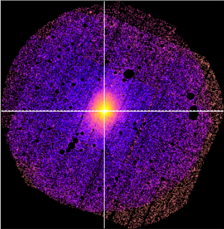
SDSSXCS-124 - Combined 0.5-2.0keV ratemapSDSSXCS-124 - Combined 0.5-2.0keV ratemap
