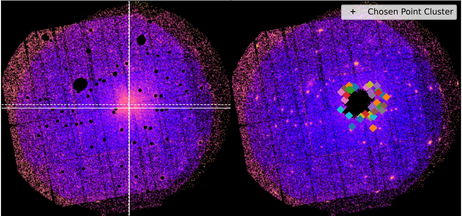
SDSSXCS-137 - Combined 0.5-2.0keV ratemapSDSSXCS-137 - Combined 0.5-2.0keV ratemap
