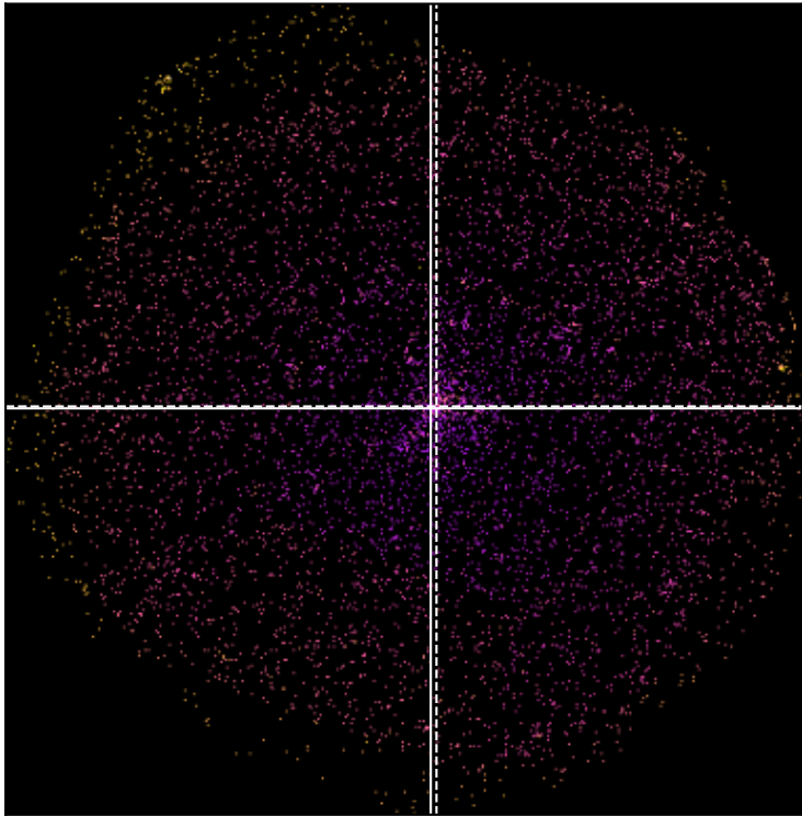
SDSSXCS-16227 - Combined 0.5-2.0keV ratemap
