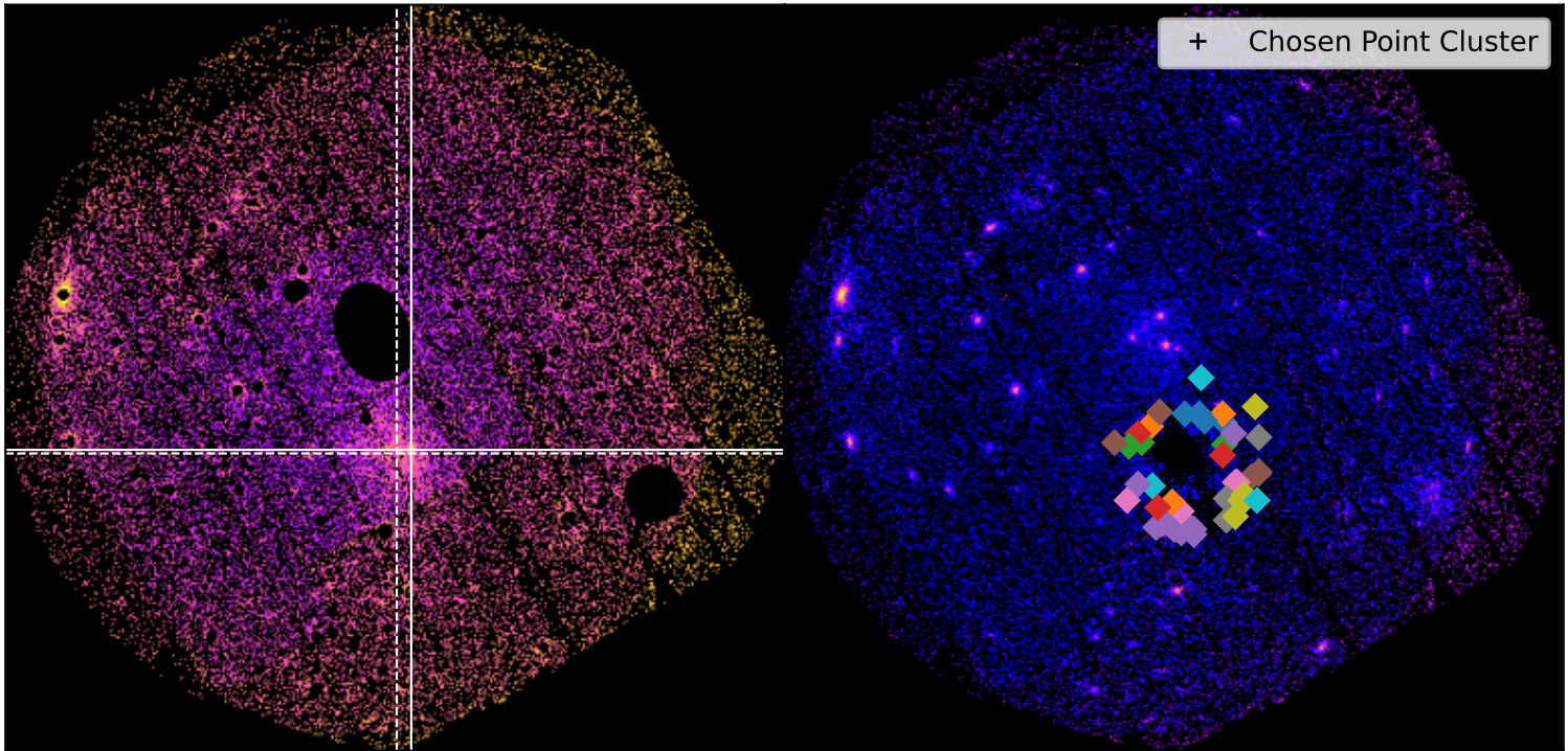
SDSSXCS-165 - Combined 0.5-2.0keV ratemapSDSSXCS-165 - Combined 0.5-2.0keV ratemap
