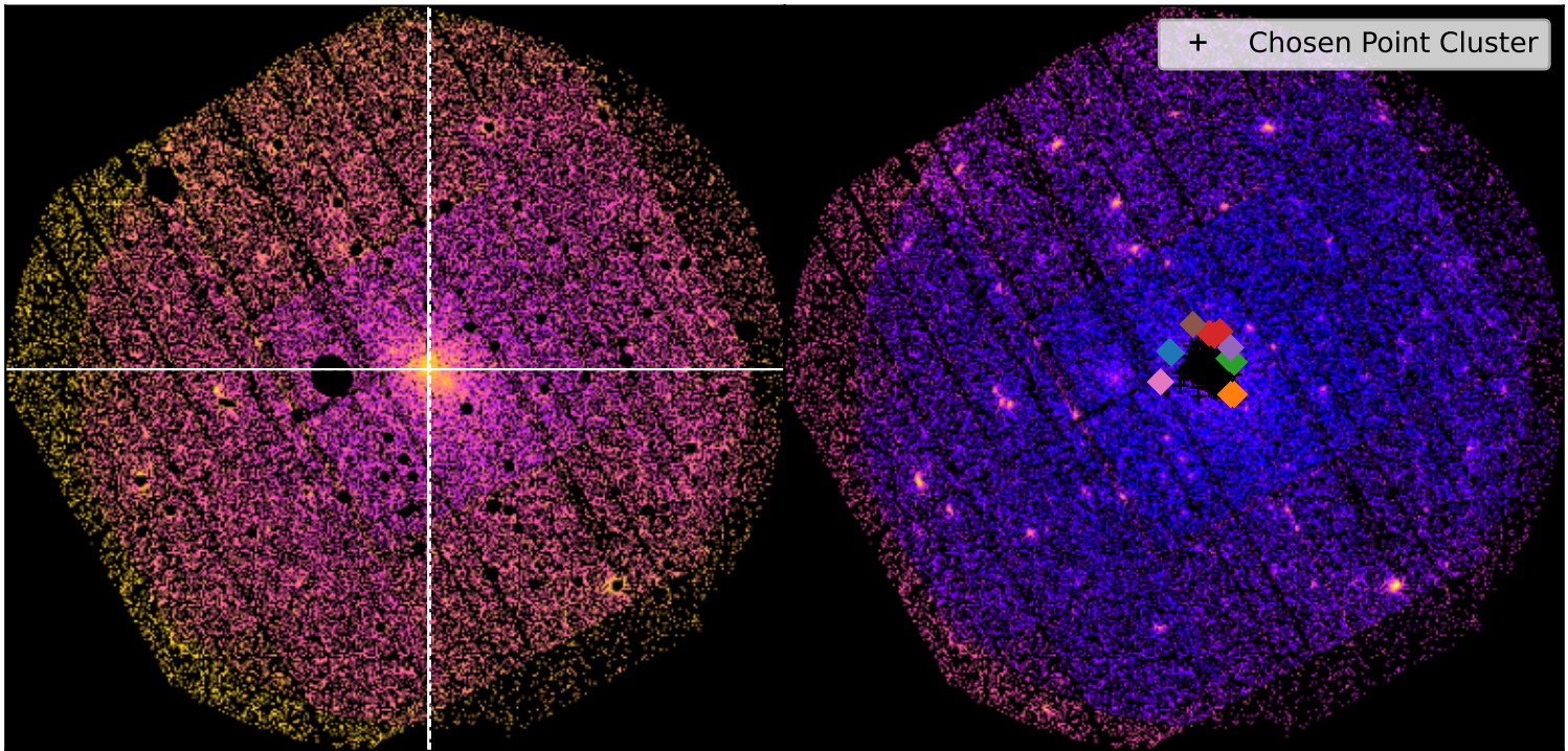
SDSSXCS-176 - Combined 0.5-2.0keV ratemapSDSSXCS-176 - Combined 0.5-2.0keV ratemap
