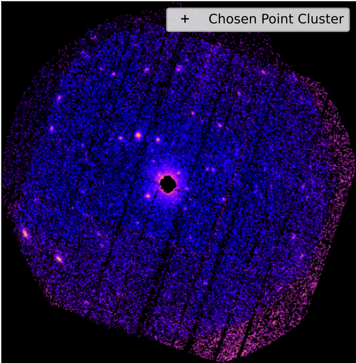
SDSSXCS-2032 - Combined 0.5-2.0keV ratemap
