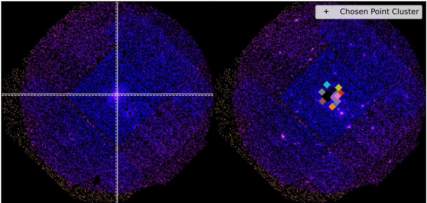
SDSSXCS-210 - Combined 0.5-2.0keV ratemapSDSSXCS-210 - Combined 0.5-2.0keV ratemap
