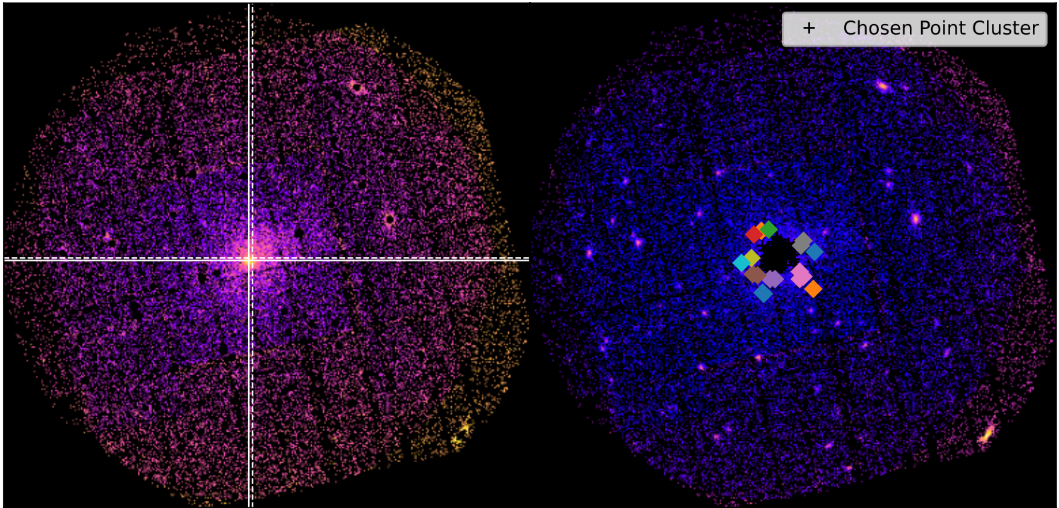
SDSSXCS-212 - Combined 0.5-2.0keV ratemapSDSSXCS-212 - Combined 0.5-2.0keV ratemap
