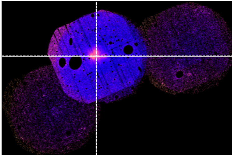
SDSSXCS-21 - Combined 0.5-2.0keV ratemap
