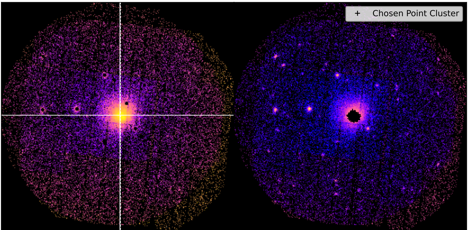
SDSSXCS-226 - Combined 0.5-2.0keV ratemapSDSSXCS-226 - Combined 0.5-2.0keV ratemap
