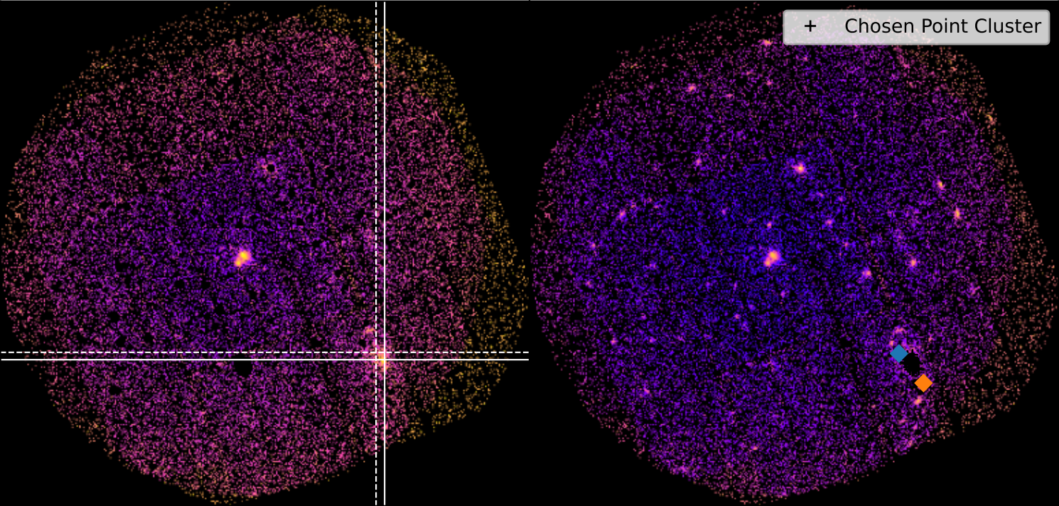
SDSSXCS-22748 - Combined 0.5-2.0keV ratemapSDSSXCS-22748 - Combined 0.5-2.0keV ratemap
