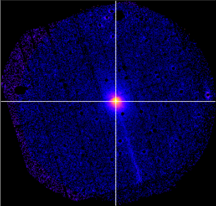
SDSSXCS-2288 - Combined 0.5-2.0keV ratemap
