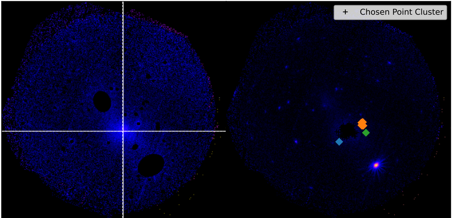
SDSSXCS-236 - Combined 0.5-2.0keV ratemapSDSSXCS-236 - Combined 0.5-2.0keV ratemap
