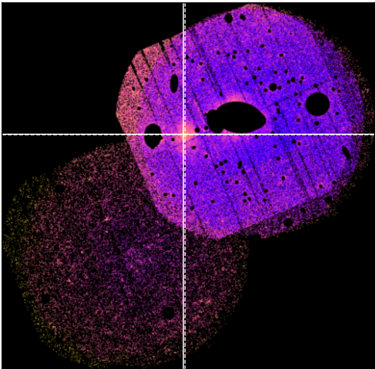
SDSSXCS-23 - Combined 0.5-2.0keV ratemap
