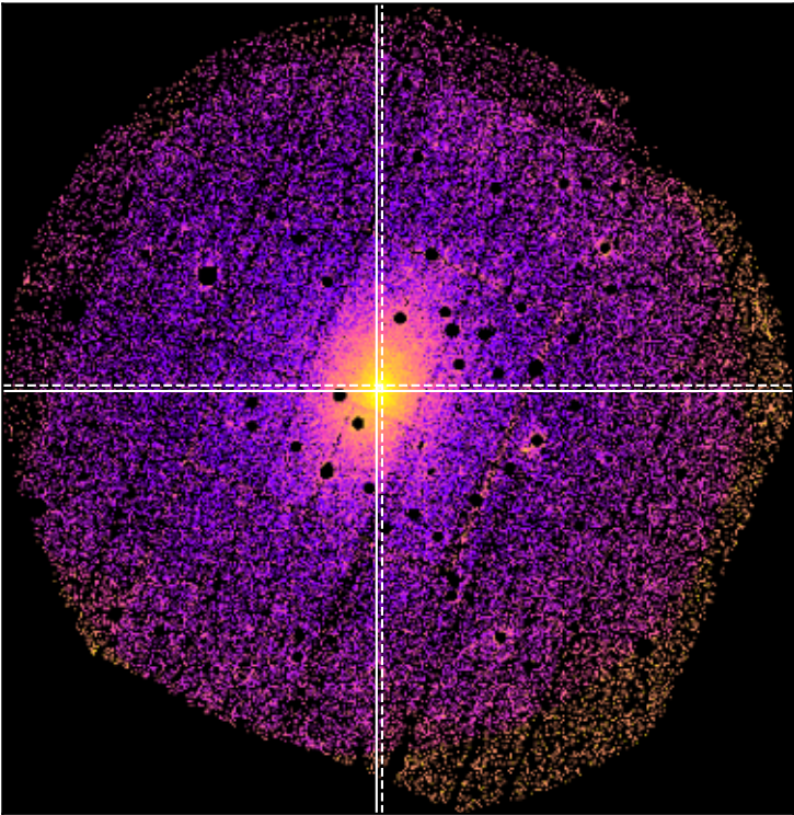
SDSSXCS-2789 - Combined 0.5-2.0keV ratemap
