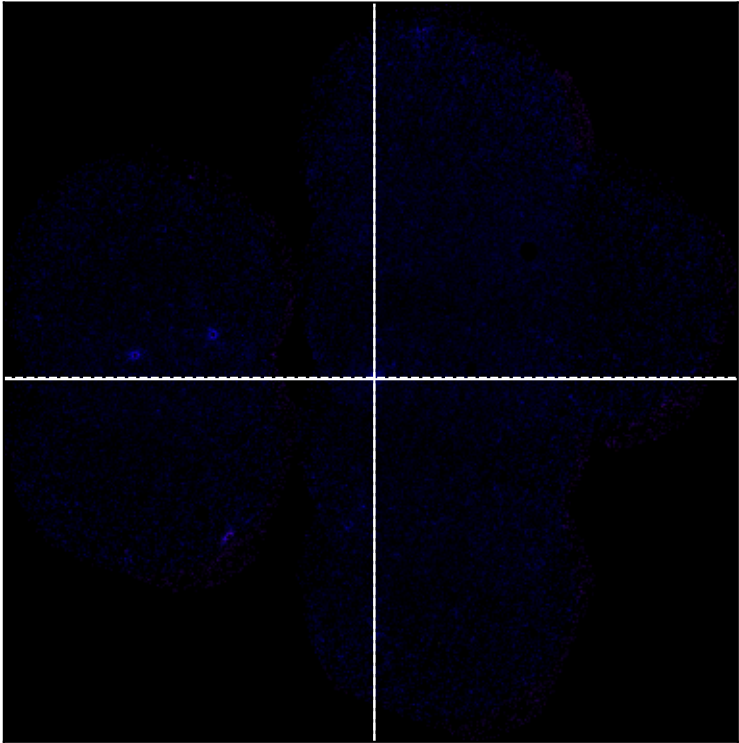
SDSSXCS-28849 - Combined 0.5-2.0keV ratemap
