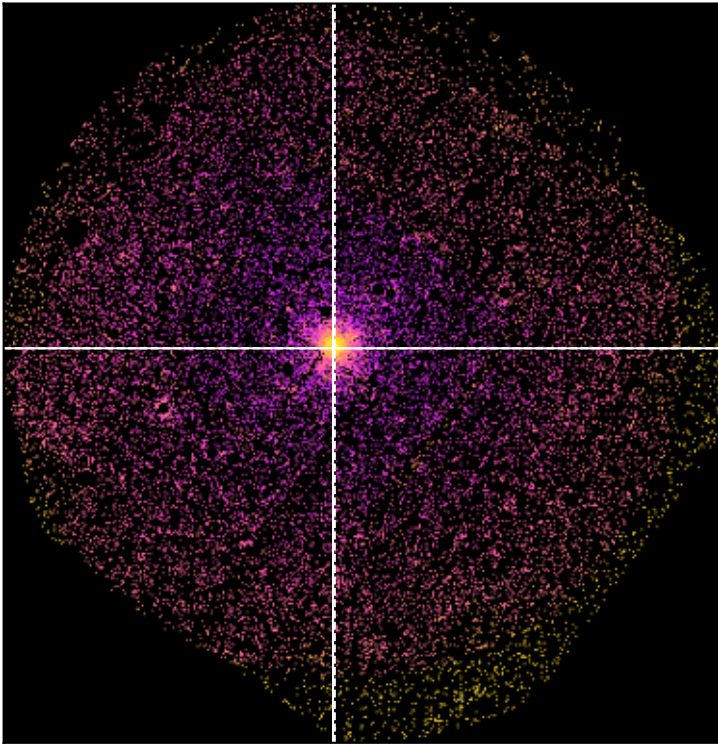
SDSSXCS-290 - Combined 0.5-2.0keV ratemapSDSSXCS-290 - Combined 0.5-2.0keV ratemap
