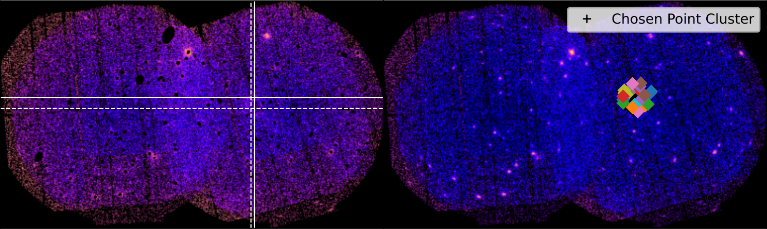
SDSSXCS-30950 - Combined 0.5-2.0keV ratemap SDSSXCS-30950 - Combined 0.5-2.0keV ratemap
