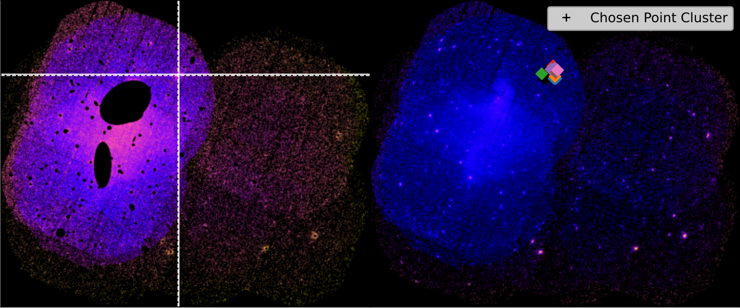
SDSSXCS-31144 - Combined 0.5-2.0keV ratemapSDSSXCS-31144 - Combined 0.5-2.0keV ratemap
