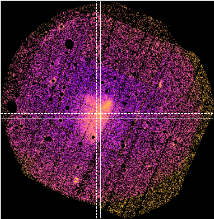
SDSSXCS-314 - Combined 0.5-2.0keV ratemapSDSSXCS-314 - Combined 0.5-2.0keV ratemap
