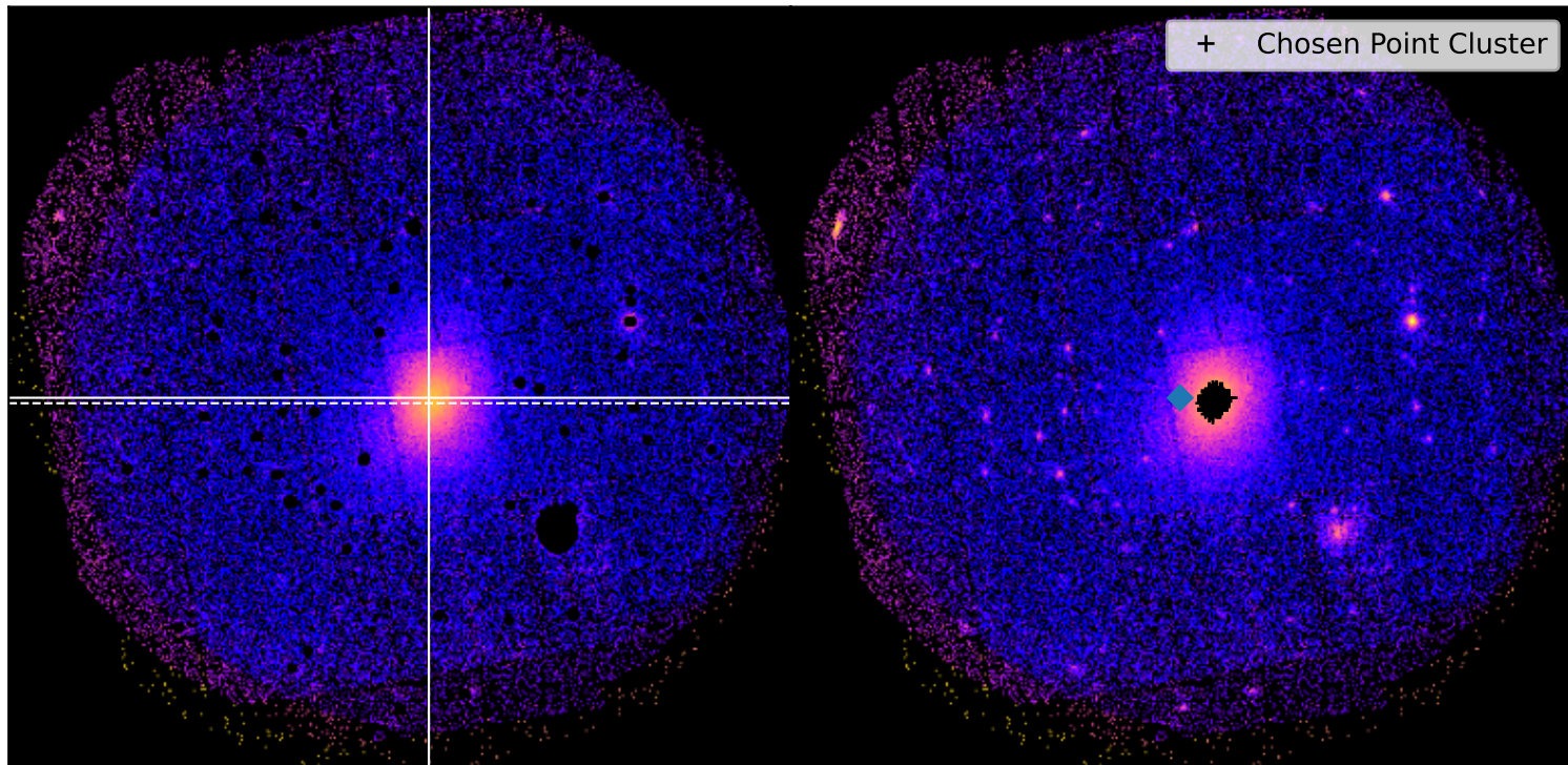
SDSSXCS-31 - Combined 0.5-2.0keV ratemap SDSSXCS-31 - Combined 0.5-2.0keV ratemap
