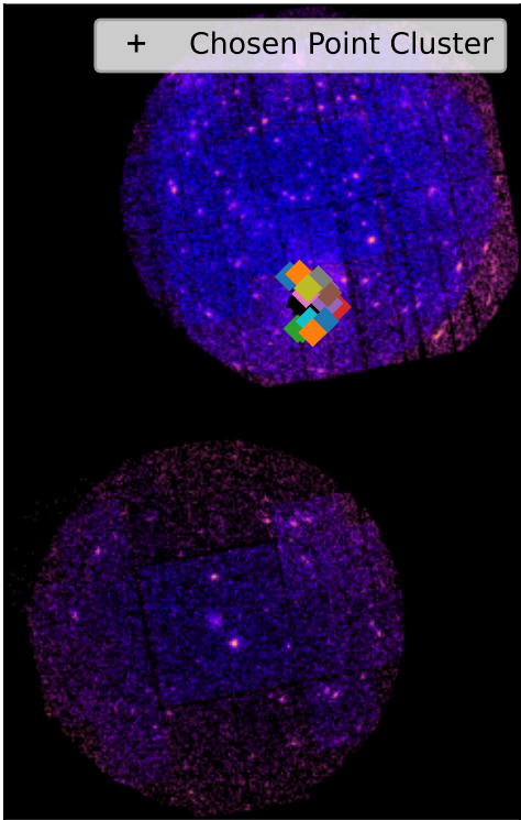
SDSSXCS-325 - Combined 0.5-2.0keV ratemapSDSSXCS-325 - Combined 0.5-2.0keV ratemap
