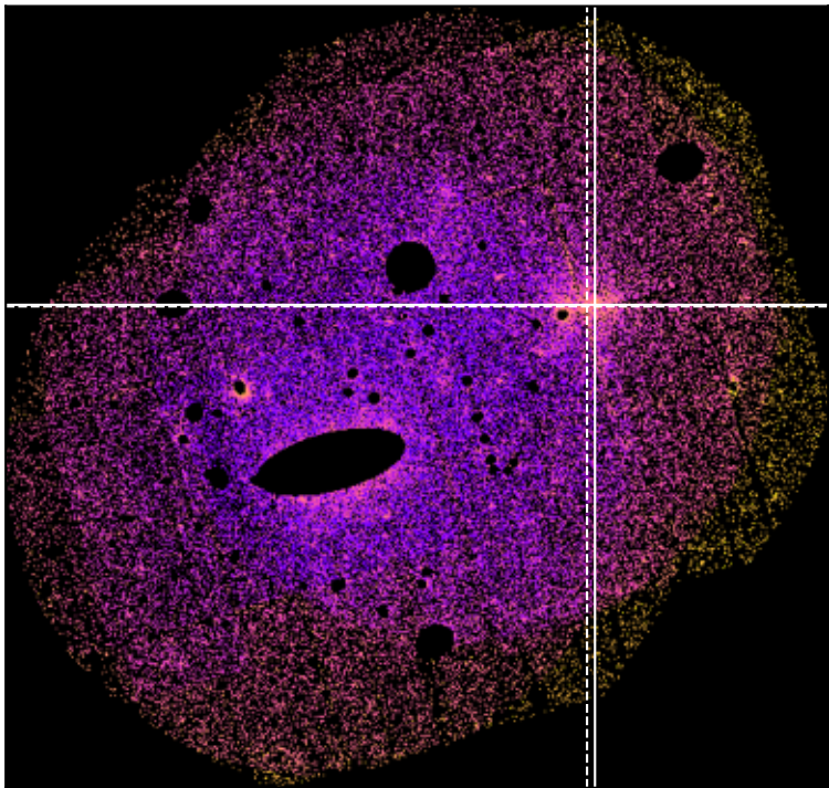
SDSSXCS-32 - Combined 0.5-2.0keV ratemap
