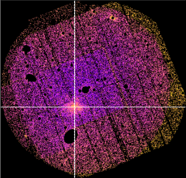
SDSSXCS-3672 - Combined 0.5-2.0keV ratemap
