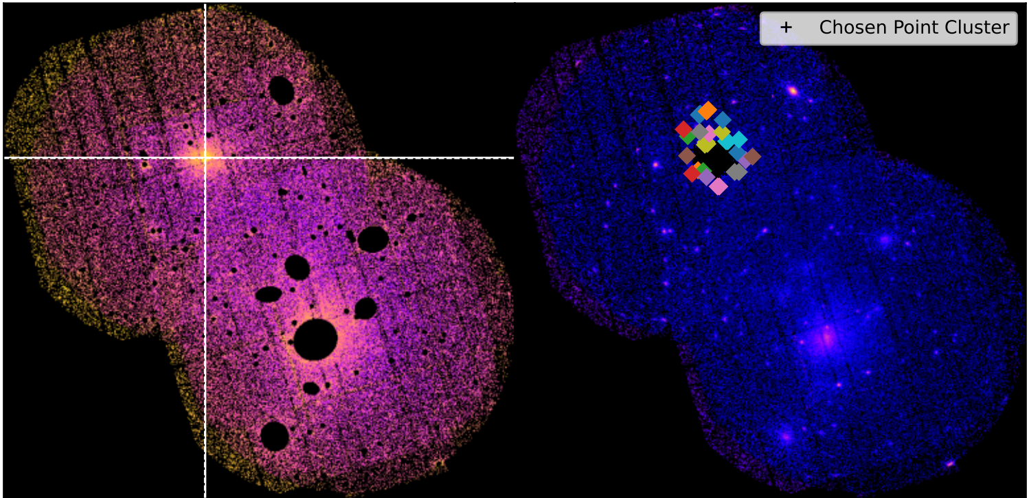
SDSSXCS-382 - Combined 0.5-2.0keV ratemapSDSSXCS-382 - Combined 0.5-2.0keV ratemap
