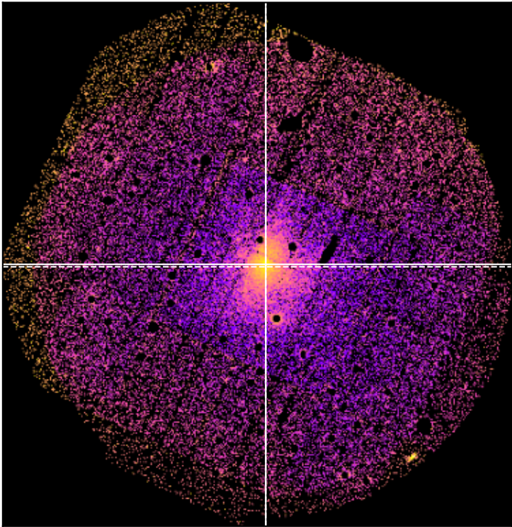
SDSSXCS-395 - Combined 0.5-2.0keV ratemapSDSSXCS-395 - Combined 0.5-2.0keV ratemap
