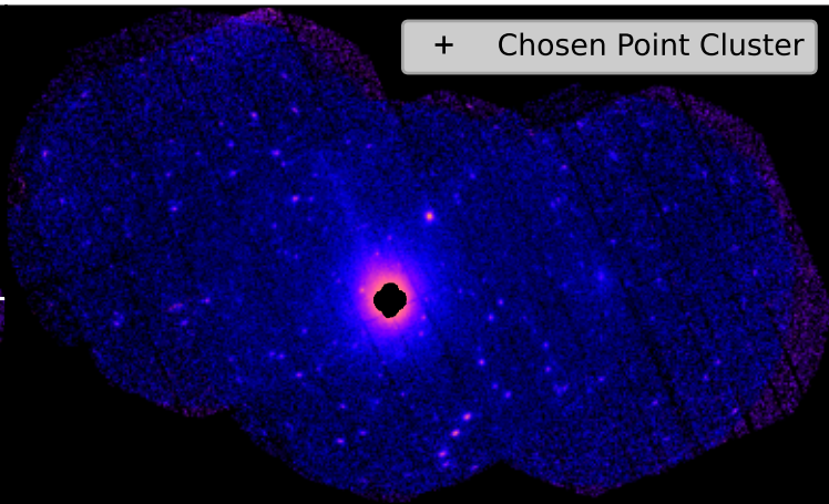
SDSSXCS-3 - Combined 0.5-2.0keV ratemap
