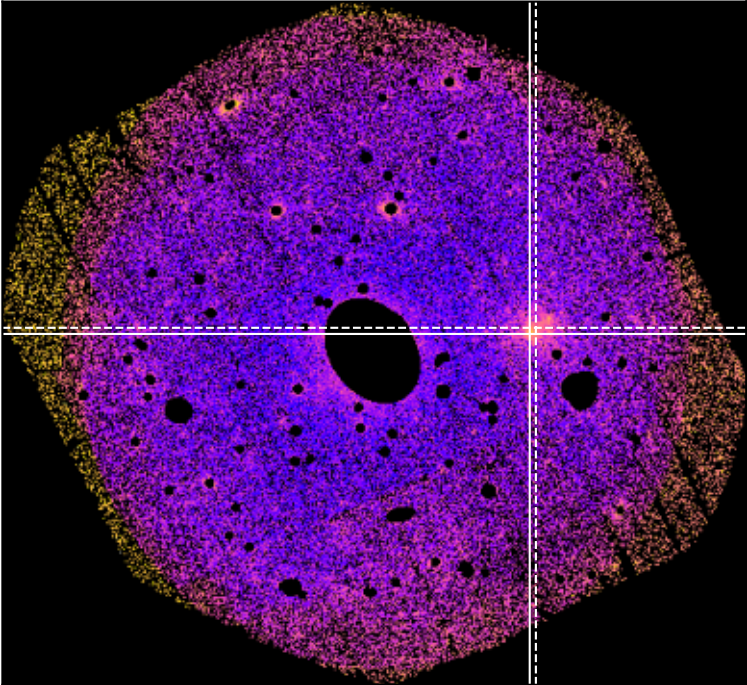
SDSSXCS-4245 - Combined 0.5-2.0keV ratemap
