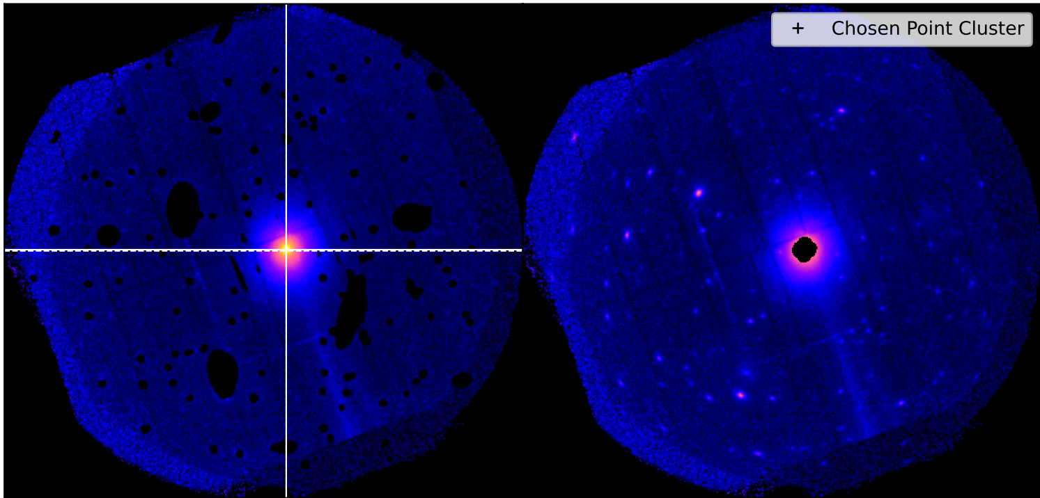
SDSSXCS-43 - Combined 0.5-2.0keV ratemap SDSSXCS-43 - Combined 0.5-2.0keV ratemap
