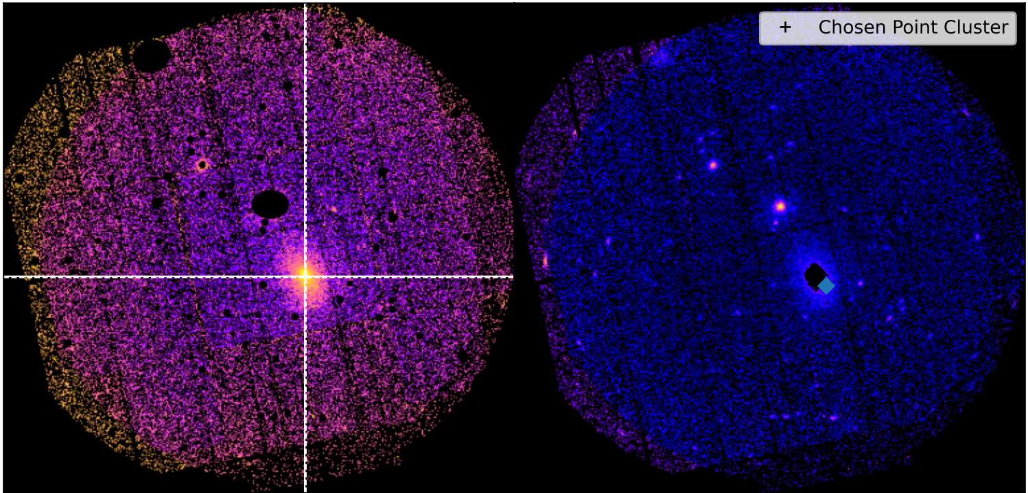
SDSSXCS-455 - Combined 0.5-2.0keV ratemapSDSSXCS-455 - Combined 0.5-2.0keV ratemap
