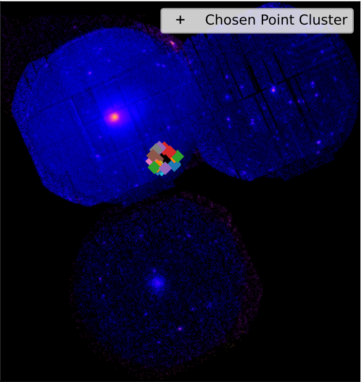
SDSSXCS-474 - Combined 0.5-2.0keV ratemapSDSSXCS-474 - Combined 0.5-2.0keV ratemap
