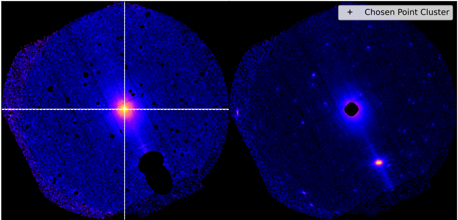
SDSSXCS-480 - Combined 0.5-2.0keV ratemapSDSSXCS-480 - Combined 0.5-2.0keV ratemap
