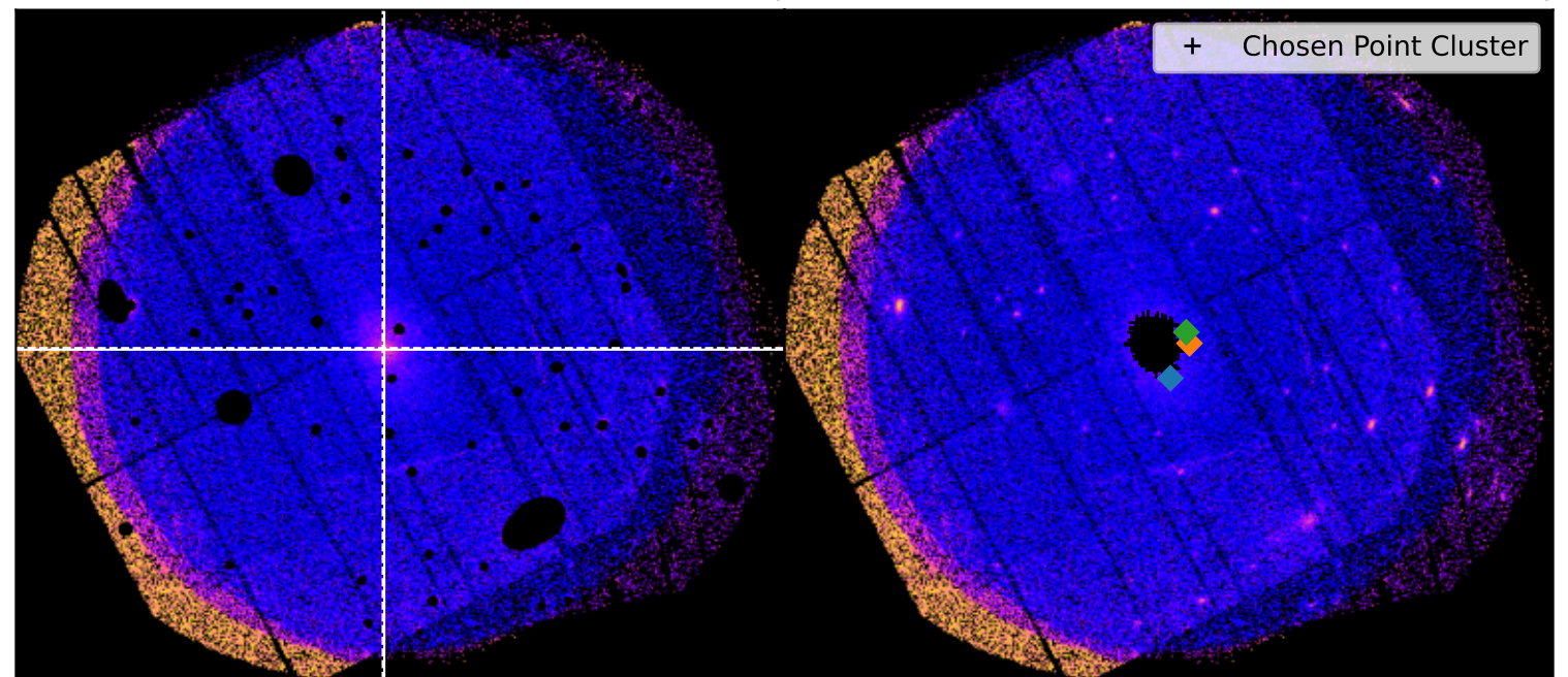
SDSSXCS-5527 - Combined 0.5-2.0keV ratemap
