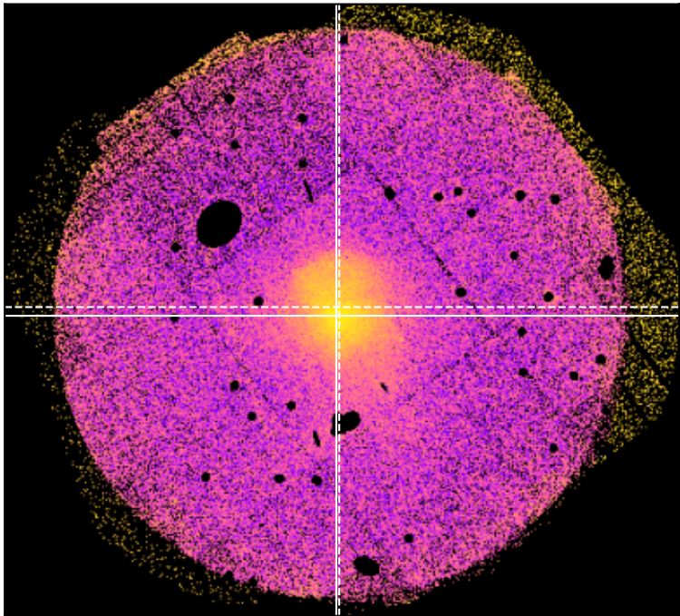
SDSSXCS-55 - Combined 0.5-2.0keV ratemap
