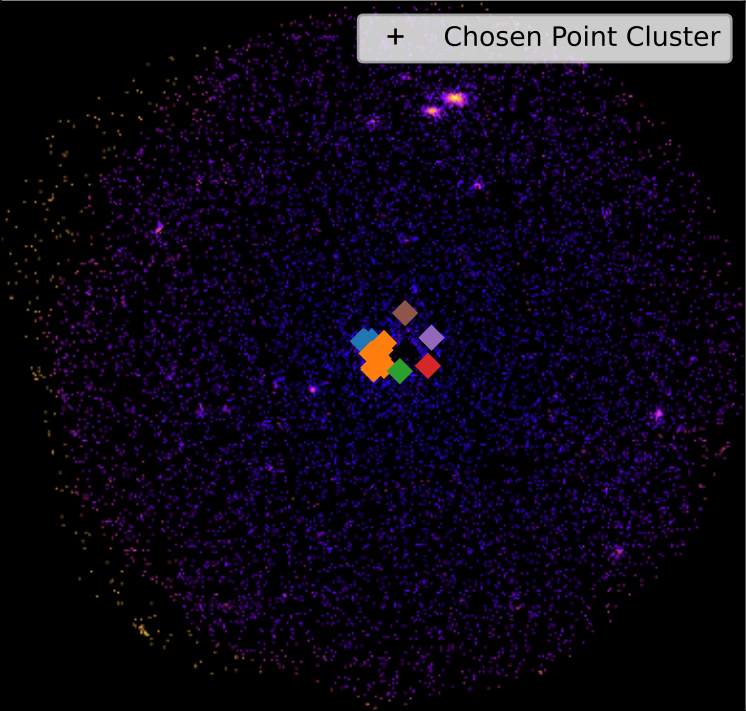
SDSSXCS-5624 - Combined 0.5-2.0keV ratemap
