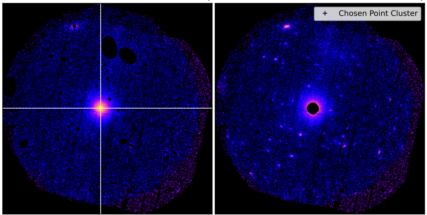
SDSSXCS-572 - Combined 0.5-2.0keV ratemapSDSSXCS-572 - Combined 0.5-2.0keV ratemap
