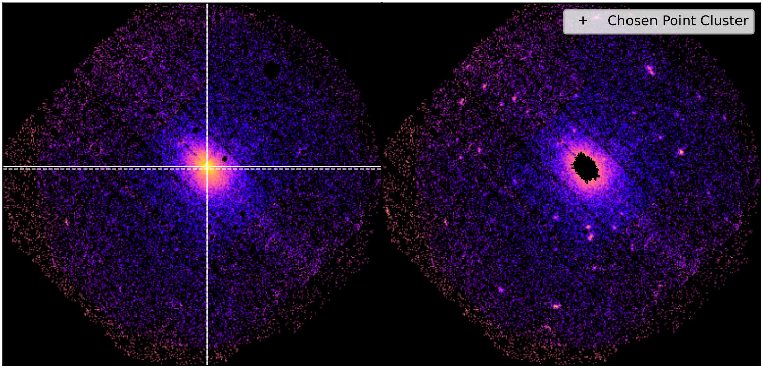
SDSSXCS-574 - Combined 0.5-2.0keV ratemapSDSSXCS-574 - Combined 0.5-2.0keV ratemap
