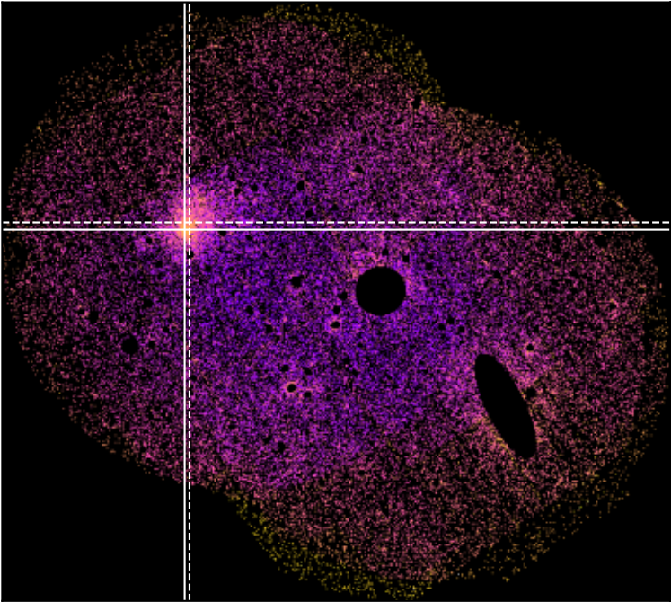
SDSSXCS-5939 - Combined 0.5-2.0keV ratemap
