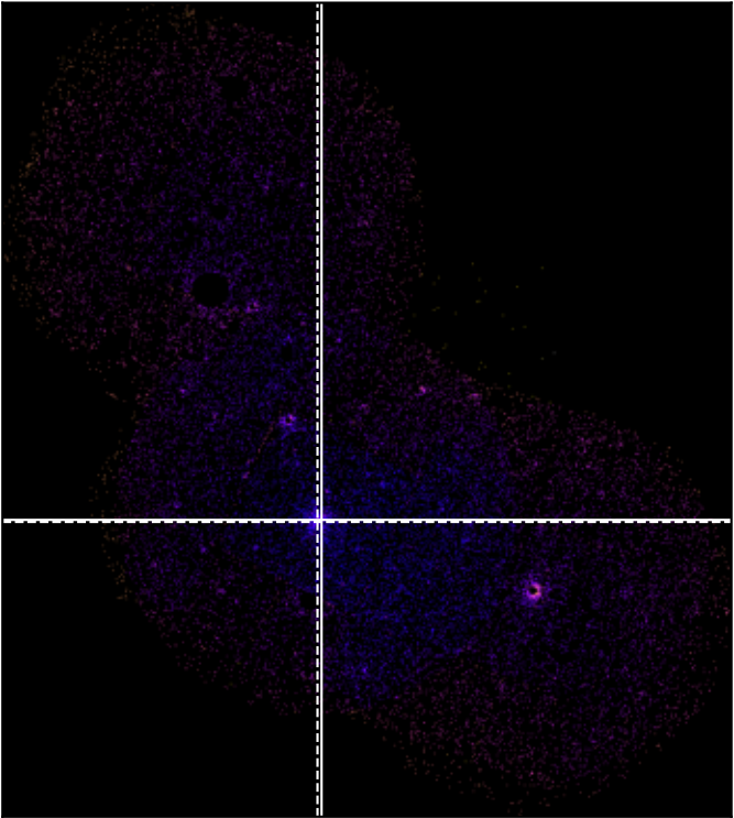
SDSSXCS-5977 - Combined 0.5-2.0keV ratemap
