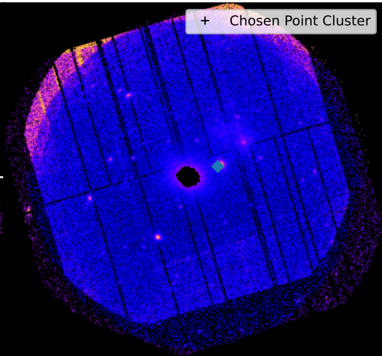
SDSSXCS-5 - Combined 0.5-2.0keV ratemap
