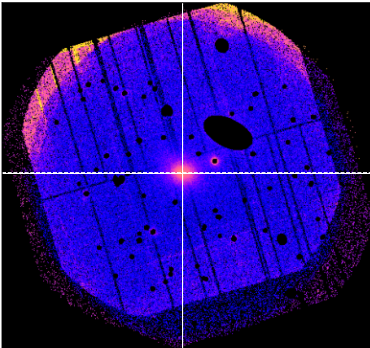
SDSSXCS-5 - Combined 0.5-2.0keV ratemap
