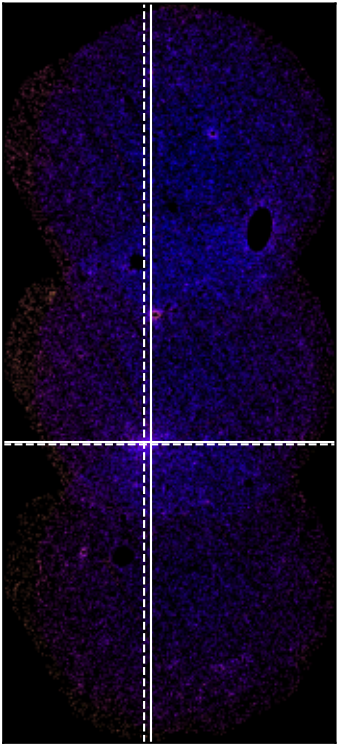
SDSSXCS-608 - Combined 0.5-2.0keV ratemapSDSSXCS-608 - Combined 0.5-2.0keV ratemap
