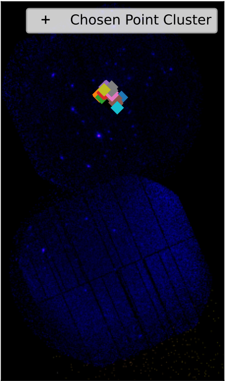
SDSSXCS-617 - Combined 0.5-2.0keV ratemapSDSSXCS-617 - Combined 0.5-2.0keV ratemap
