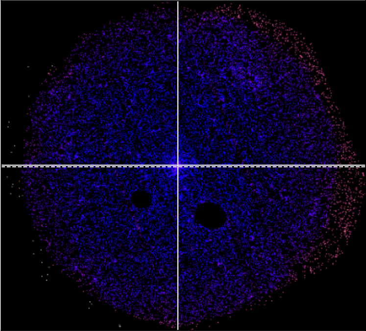
SDSSXCS-6245 - Combined 0.5-2.0keV ratemap
