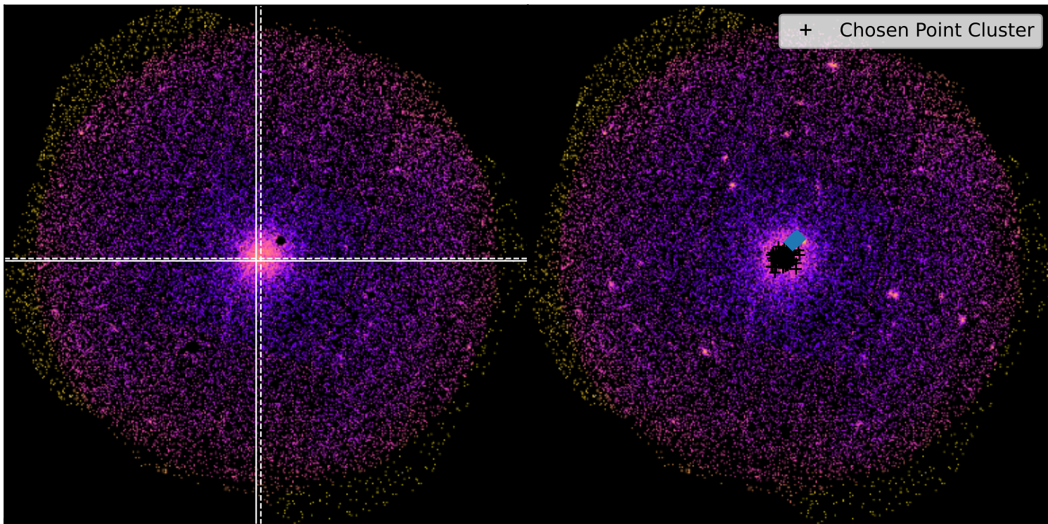
SDSSXCS-62 - Combined 0.5-2.0keV ratemap SDSSXCS-62 - Combined 0.5-2.0keV ratemap
