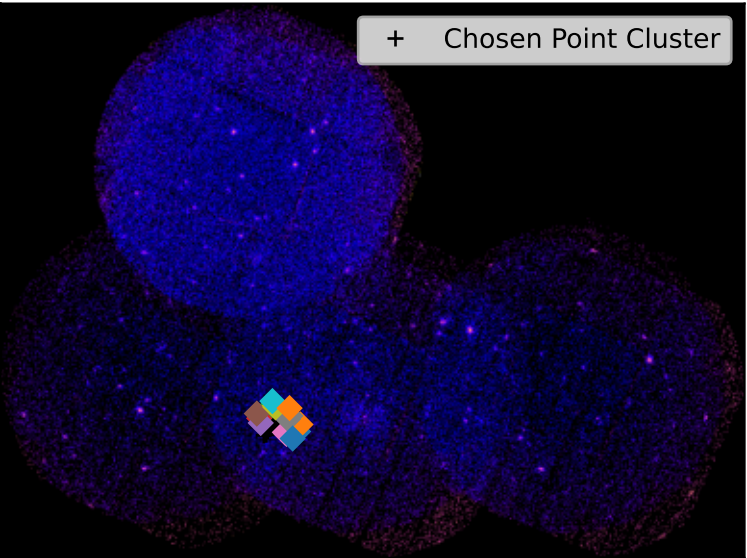
SDSSXCS-6955 - Combined 0.5-2.0keV ratemap
