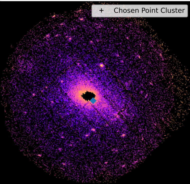
SDSSXCS-6 - Combined 0.5-2.0keV ratemap
