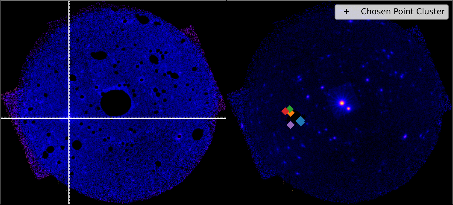
SDSSXCS-7416 - Combined 0.5-2.0keV ratemapSDSSXCS-7416 - Combined 0.5-2.0keV ratemap
