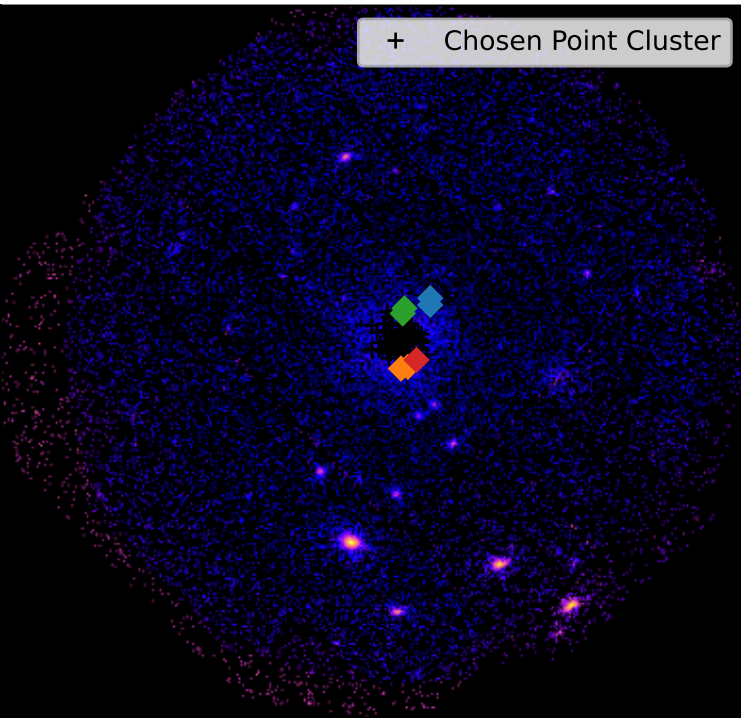
SDSSXCS-75 - Combined 0.5-2.0keV ratemap
