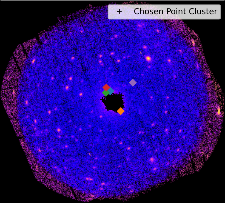
SDSSXCS-8060 - Combined 0.5-2.0keV ratemap
