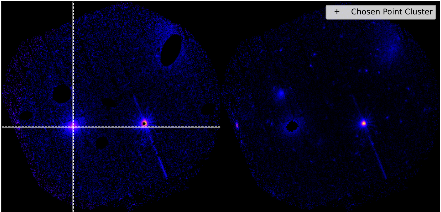
SDSSXCS-890 - Combined 0.5-2.0keV ratemapSDSSXCS-890 - Combined 0.5-2.0keV ratemap
